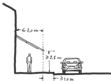
Figure 2 : Saillies mobiles
